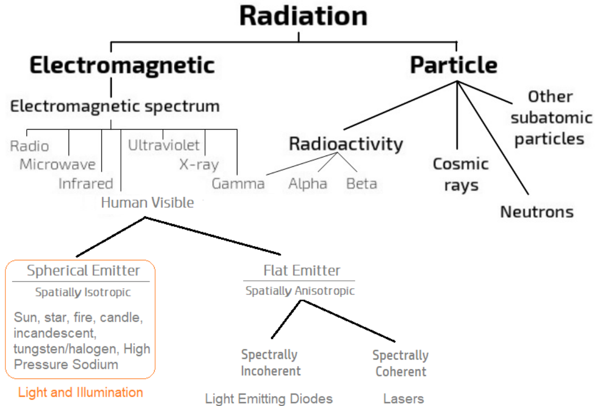
Figure 1 - Radiation Types
