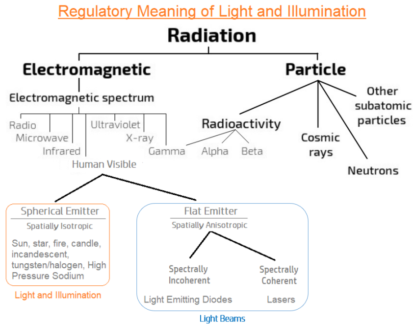
Figure 3 - Radiation Types
