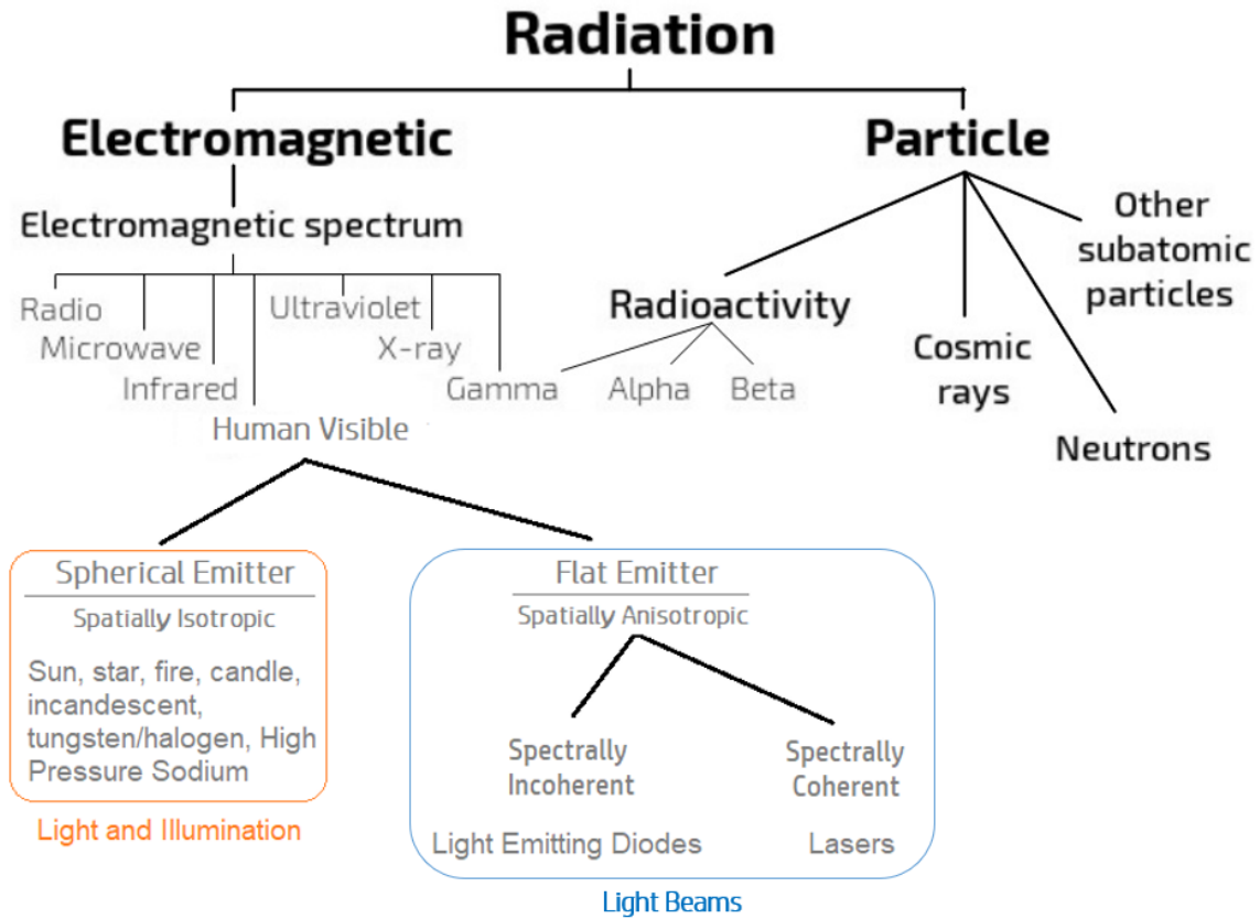
Figure 3 - Radiation Types
