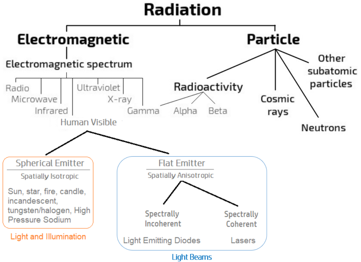
Figure 3 - Radiation Types
