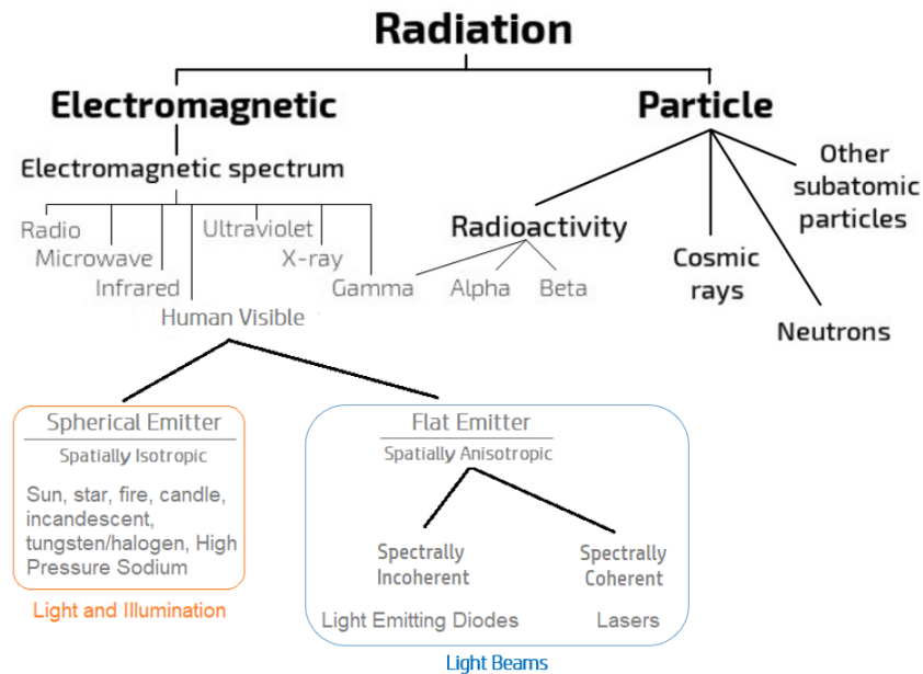
Figure 4 - Radiation Types
