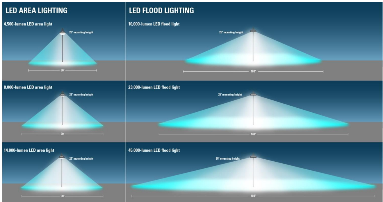
Figure 2 - LED Non-Uniform Light Distribution
