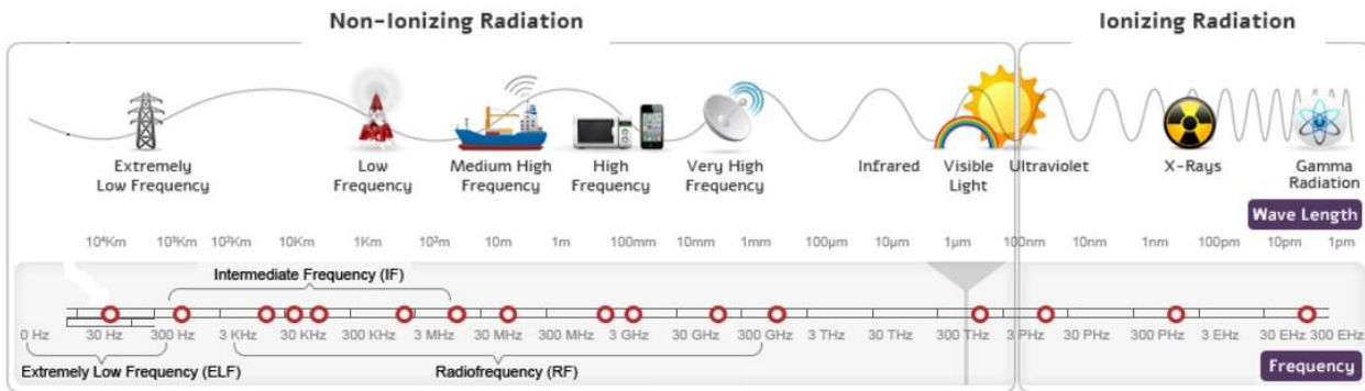
Figure 5 - Electromagnetic Spectrum 14
