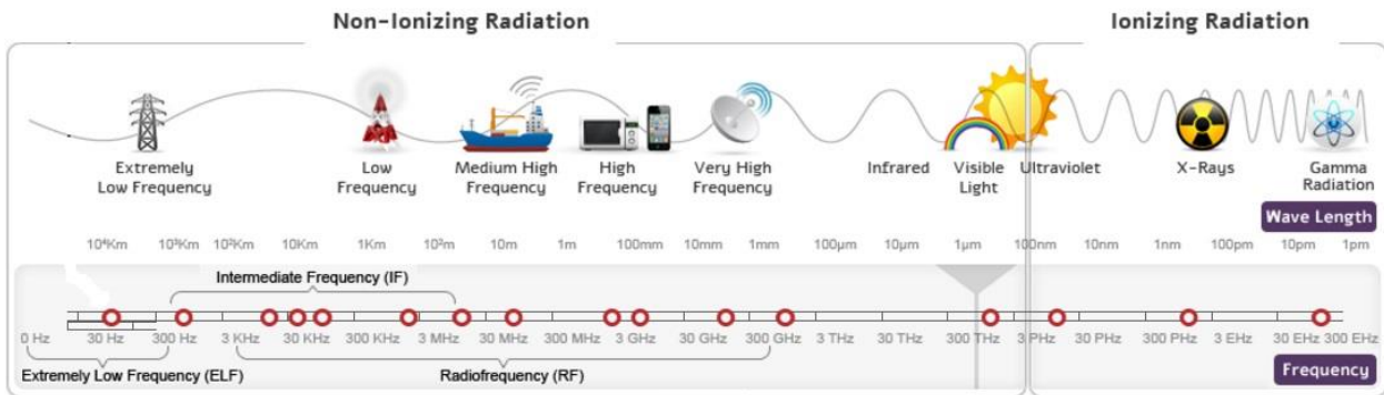
Figure 5 - Electromagnetic Spectrum 14
